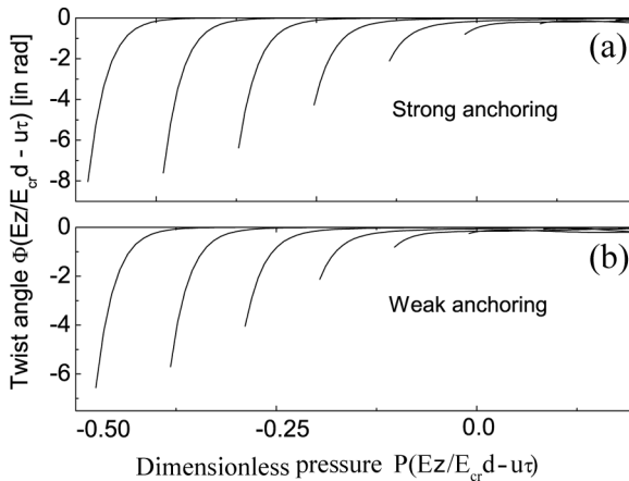
FIGURE 5 (a) Pressure P(Ez/E_{cr}d - u\tau) shape evolution from the one edge ( z/d = 0.5 ) of the cell to the second edge ( z/d = -0.5 ), calculated using Eq. (7), with the boundary conditions (5), and under action of the electric field E/E_{cr} = 10 and (A\kappa/2K_2)\sin 2\Delta\phi = 1 . The initial condition of twist angle is the same as Figure 1(a); (b) Same as (a), but with the boundary conditions (6).
