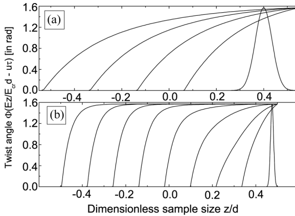
FIGURE 2 (a) Wave shape evolution of the azimuthal angle \phi(Ez/E_{\text{cr}}d - u_r) from the upper edge ( z/d = 0.5 ) of the cell to bottom edge ( z/d = -0.5 ) calculated using Eq. (4), with the boundary conditions (6), at (A\kappa/2K_2)\sin 2\Delta\phi = 1.0 and under action of the electric field E/E_{\text{cr}} = 2.2 . The initial condition is \phi(\tau = 0, q) = \varphi((q - q_3)/\sigma) , where q_3 = 0.9 and \sigma = 0.05 which correspond to z_3 = 0.4 and \sigma_z = 0.023 at static scale z/d ; (b) The same as (a), but E/E_{\text{cr}} = 10 , with the initial condition as Figure 1(a).
