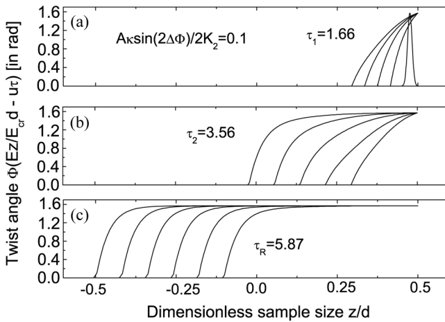
FIGURE 3 Plot of three stages of the director evolution in the TN cell, calculated using Eq. (4), with the boundary conditions (6), at (A\kappa/2K_2)\sin 2\Delta\phi = 0.1 and E/E_{cr} = 10 . The initial condition of twist angle is the same as Figure 1(a).
